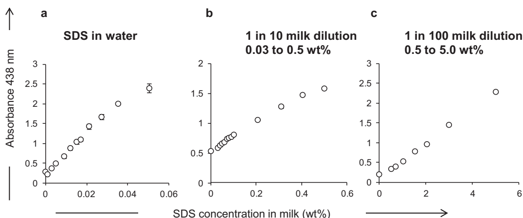
Fig. 3. Simple, rapid measurement of SDS concentration in milk using stains-all dye. The absorbance at 438 nm was measured for known concentrations of SDS dissolved either in (a) water or milk subsequently diluted in (b) 1:10 water dilution or (c) 1:100 water dilution. A clear linear relationship between absorbance and SDS concentration is apparent for each fixed dilution ratio allowing accurate measurement of SDS release into milk over a range of concentrations. Data representative of >20 experiments; fresh standard curves were prepared for every release experiment using the same batch and type of milk tested to determine SDS concentrations. The standard error of repeat measurements is displayed.
