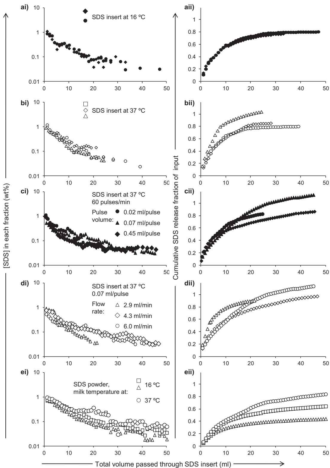
Fig. 4. Effect of SDS form, temperature and flow on release kinetics. Pasturised cow's milk was flowed through SDS loaded onto non-woven fiber discs (a–d) or SDS powder (e) and SDS concentration determined. (a, b) The effect of temperature on release at a flow rate of 4.3 ml/min and pulse rate 60 pulses/min was determined. (c) The effect on release of varying pulse volume at a fixed pulse rate of 60 pulses/min was determined. (d) The effect of varying pulse rate for a fixed pulse volume of 0.07 ml/min was determined. (e) The release of SDS in powder form at 16 °C and 37 °C at a flow rate of 4.3 ml/min and pulse rate 60 pulses/min was measured. Data displayed as (i) concentration of SDS in individual collected 1 ml fractions and (ii) cumulative SDS release relative to input SDS load. In all cases, each set of symbols represents an individual release experiment, with the mean of triplicate measurements of SDS concentrations for each fraction shown.
