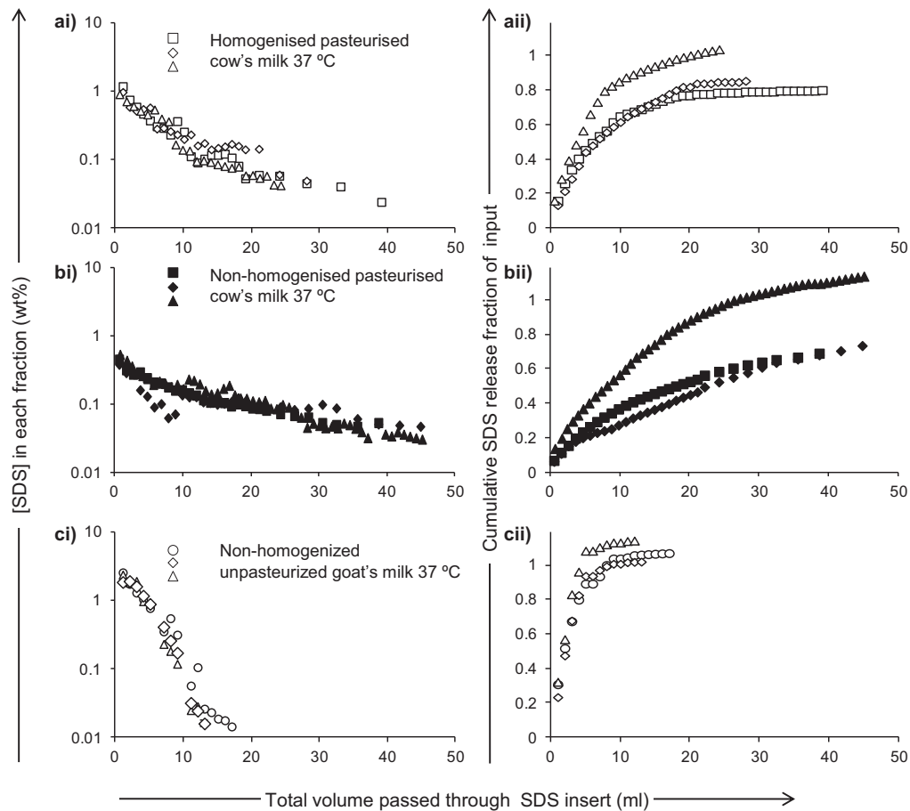
Fig. 5. Effect of milk type on SDS release kinetics. The release of SDS from loaded non-woven fiber discs during pulsed flow into (a) homogenised pasteurised cow's milk, (b) non-homogenised cow's milk and (c) non-homogenised unpasteurised goat's milk was measured with a flow rate of 4.3 ml/min and pulse rate of 60/min. Data are displayed as concentration of SDS in collected 1 ml fractions (i) and cumulative SDS release relative to input disc load (ii). In all cases, each set of symbols represents an individual release experiment, with the mean of triplicate measurements of SDS concentrations for each fraction shown.
